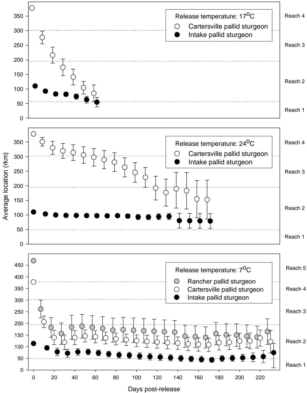
Figure 3. Distributions of telemeasured juvenile pallid sturgeon stocked in the Yellowstone River at 7, 17, and 24°C at 10-day intervals post-release. Circles represent mean river location and whiskers represent 95% confidence intervals. River location describes the distance from the confluence with the Missouri River.
